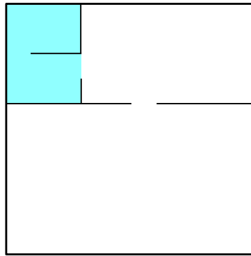
Figure 363: How the Recursive Division Algorithm Works (3/6)
